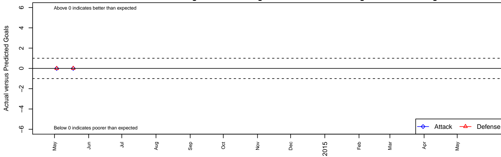
QC Fusion B99 Dots are actual minus expected GF (blue circles) and GA (red triangles). Blue line is smoothed change in attack strength. Red is smoothed change in defense strength.
